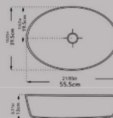
Top Counter Basin Ellipse JUPITER Without Tap Hole Built in
