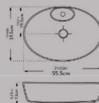
Top Counter Basin Ellipse JUPITER With Tap Hole Built in
