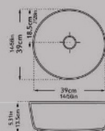
Countertop Basin Circle JUPITER Without Tap Hole Built in
