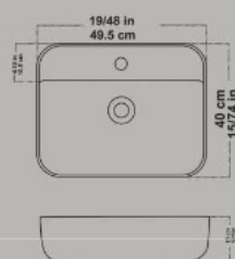
Top Counter Basin G.S.F Tap head
