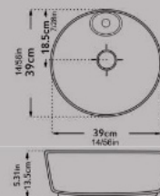
Countertop Basin Circle JUPITER With Tap Hole Built in
